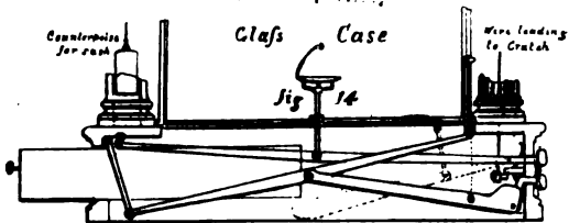
Section of Pedestal.
